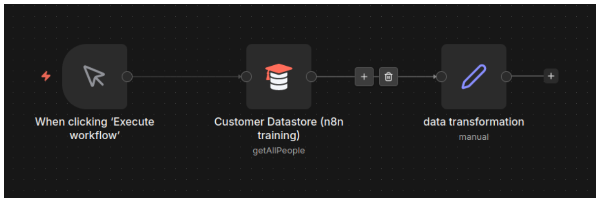
Figure 5: Simple workflow
